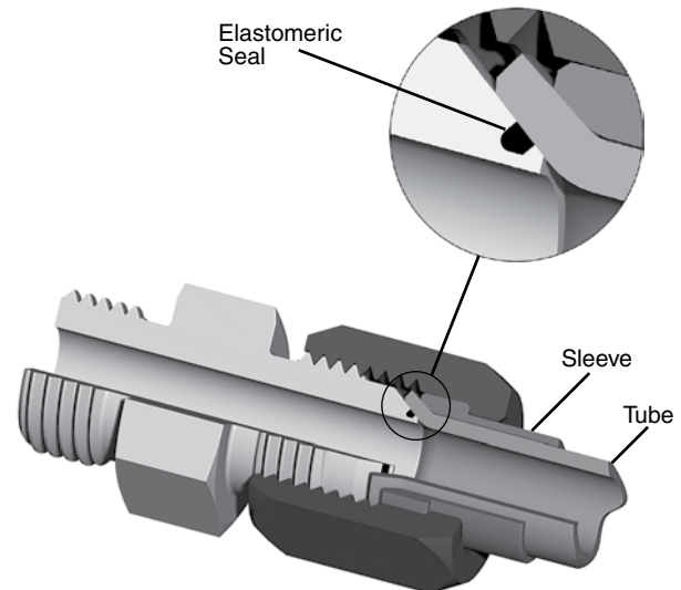
Fig. B3 – Triple-Lok 2 Design and Features
